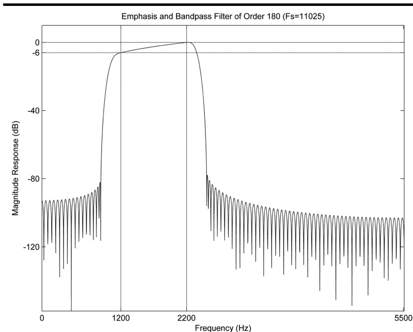
Figure 2 — Here is the response of the 900 to 2500 Hz high order (180) bandpass filter I created in Matlab . Note the 6 dB ramp up of the response across the passband, so there is no gain or attenuation at 2200 Hz.
